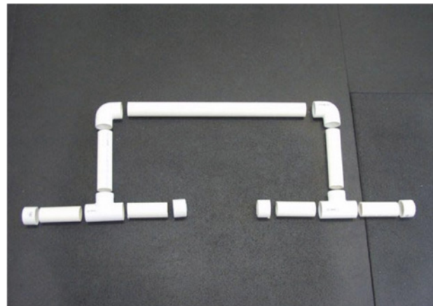
Pre-assembly check.
